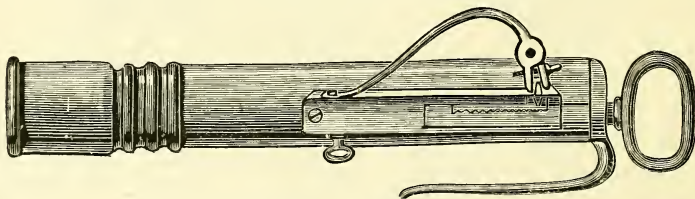
The "Monk's Gun," 1510-15.
